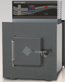
MUFFLE FURNACE Temp. Range : 930°C / 1150°C
